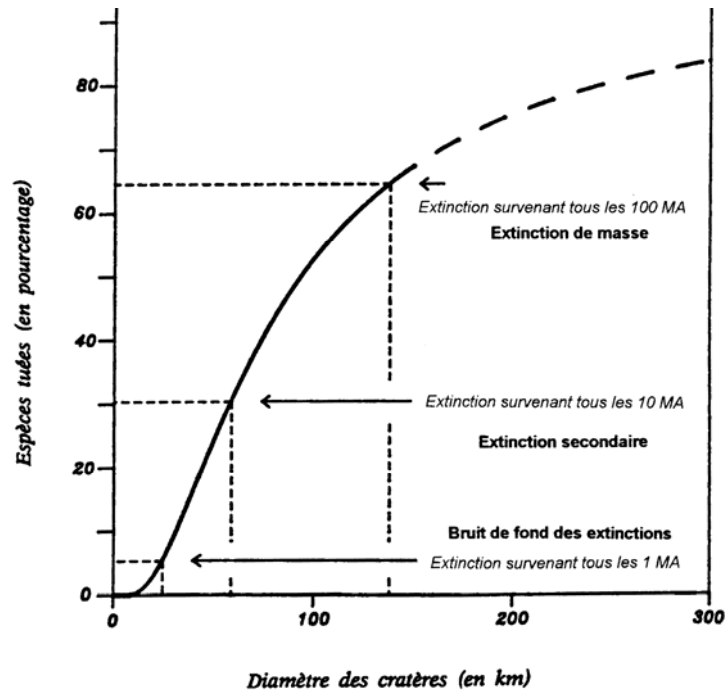
Figure 15-5. Courbe extinctions-impacts
