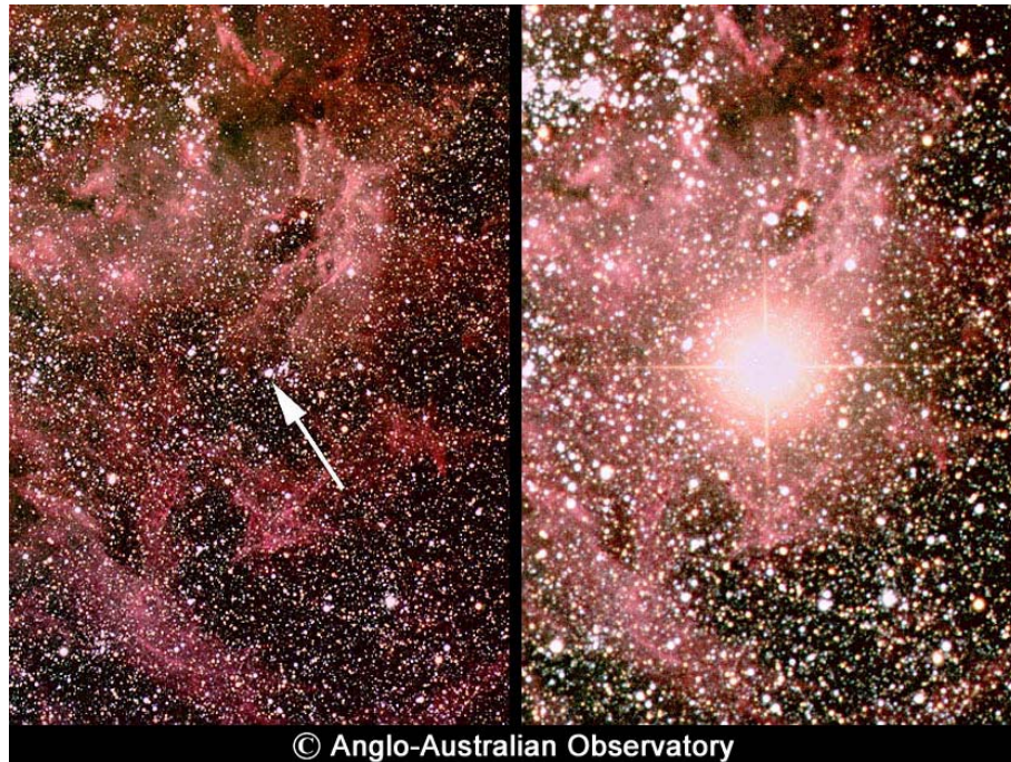
Figure 5-8. La supernova de 1987 (SN 1987A)
